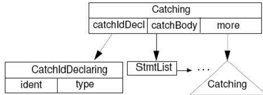
Figure 9.25: Abstract Syntax Tree for a Catch Block
