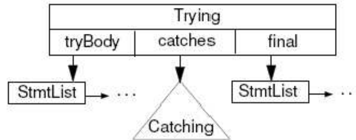
Figure 9.24: Abstract Syntax Tree for a Try Statement
