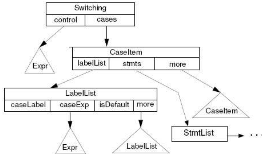
Figure 9.20: Abstract Syntax Tree for a Switch Statement
