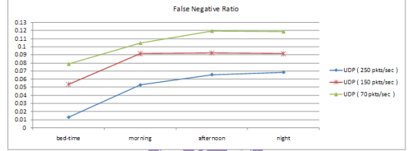
Figure 8. False negative ratio in UDP flooding.
